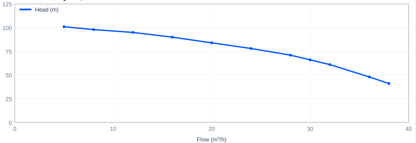
Head versus flow - PQ30-9, 50 Hz
