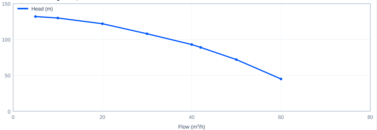
Head versus flow - PQ42-10, 50 Hz
