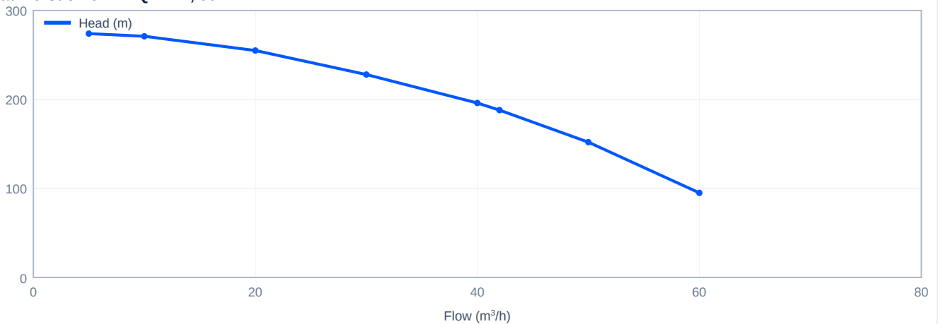
Head versus flow - PQ42-21, 50 Hz
