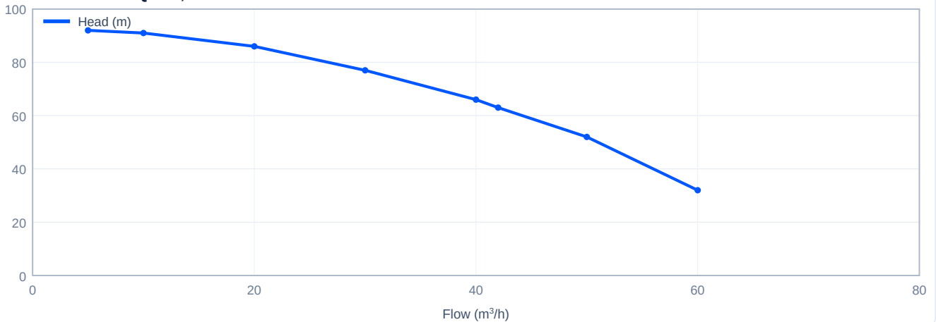
Head versus flow - PQ42-7, 50 Hz
