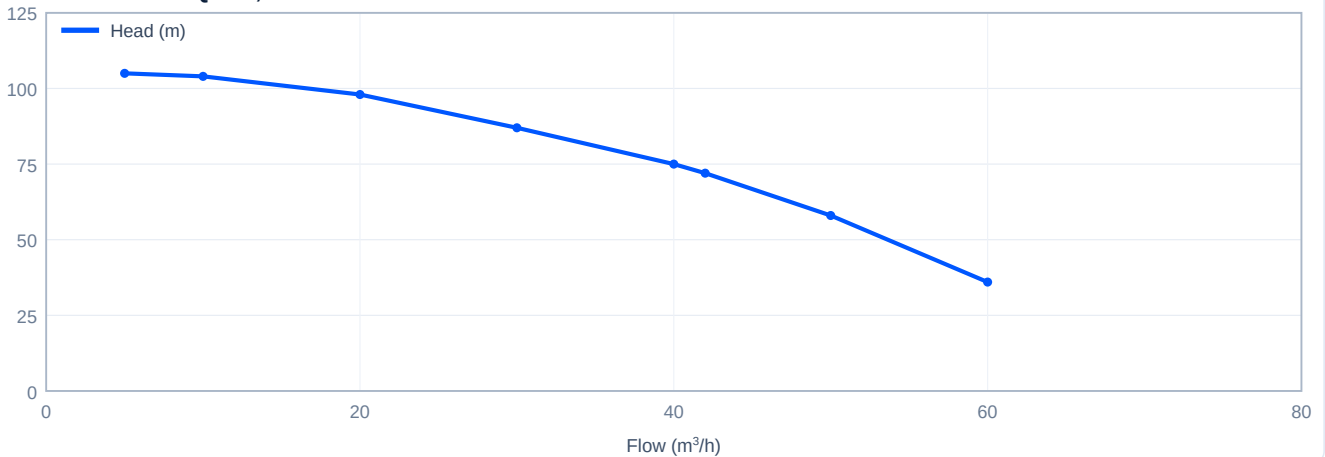
Head versus flow - PQ42-8, 50 Hz
