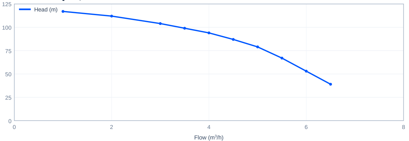
Head versus flow - PQ5-21, 50 Hz
