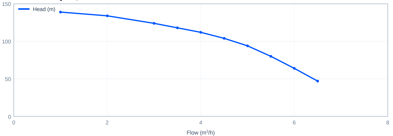
Head versus flow - PQ5-25, 50 Hz
