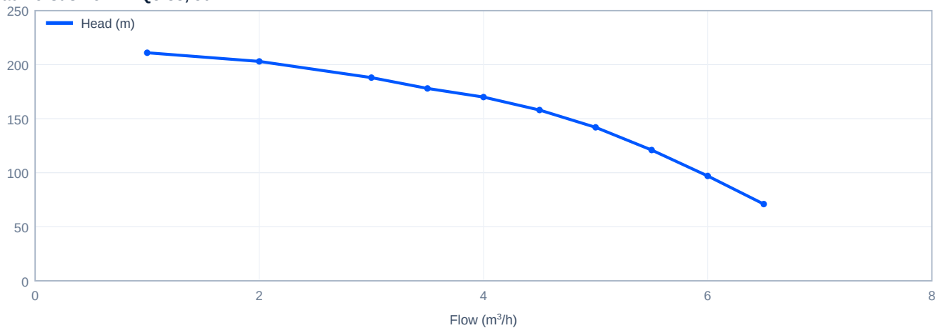
Head versus flow - PQ5-38, 50 Hz
