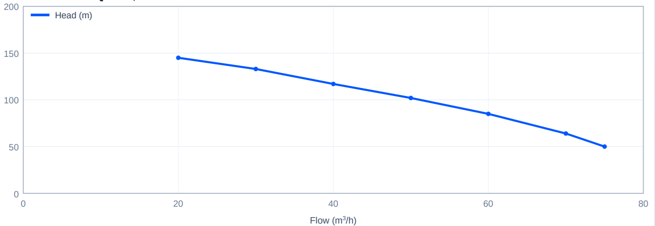
Head versus flow - PQ60-11, 50 Hz
