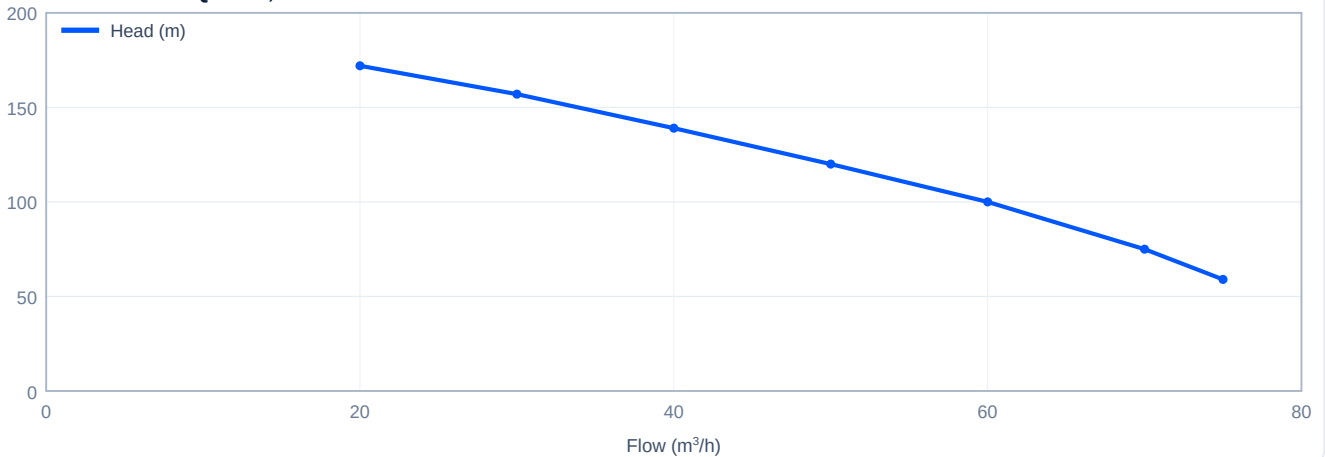
Head versus flow - PQ60-13, 50 Hz
