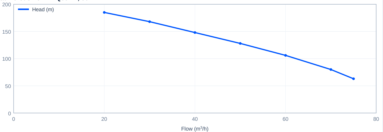
Head versus flow - PQ60-14, 50 Hz
