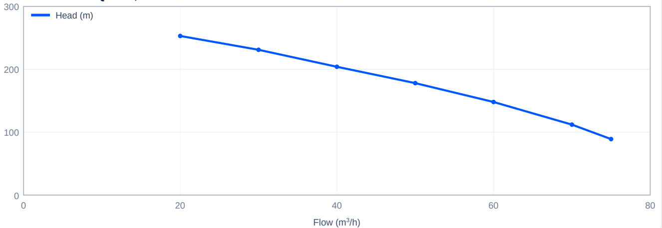
Head versus flow - PQ60-19, 50 Hz
