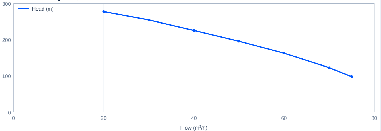
Head versus flow - PQ60-21, 50 Hz
