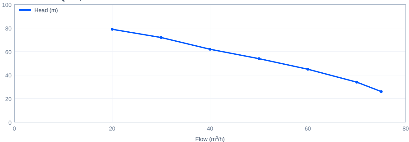
Head versus flow - PQ60-6, 50 Hz
