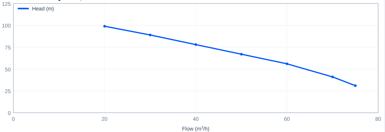
Head versus flow - PQ60-8-2, 50 Hz
