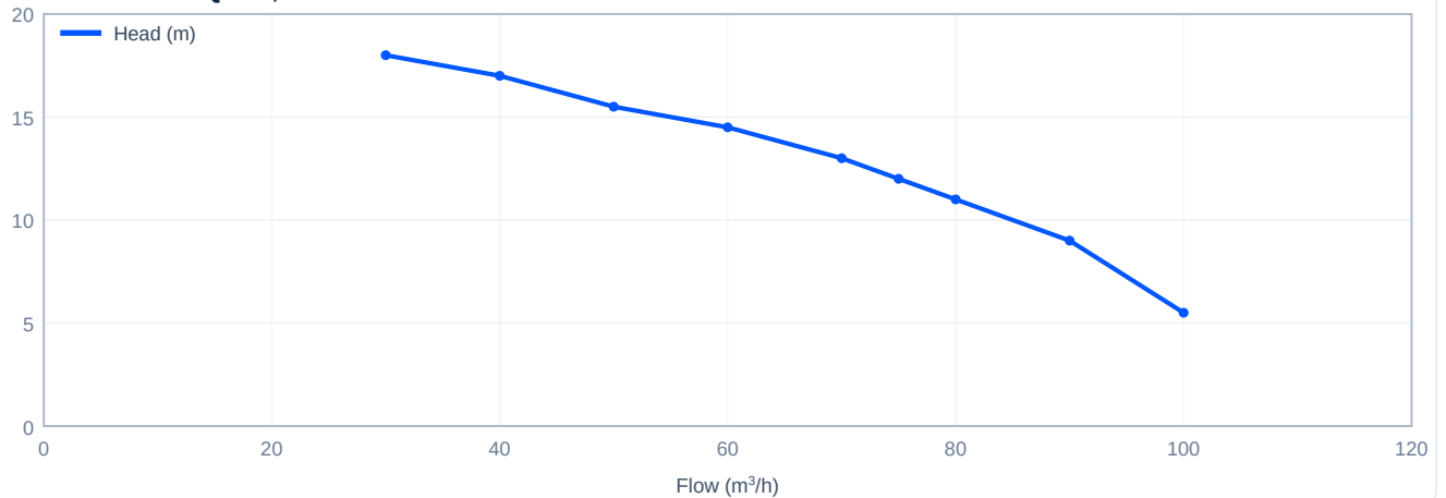
Head versus flow - PQ75-1, 50 Hz
