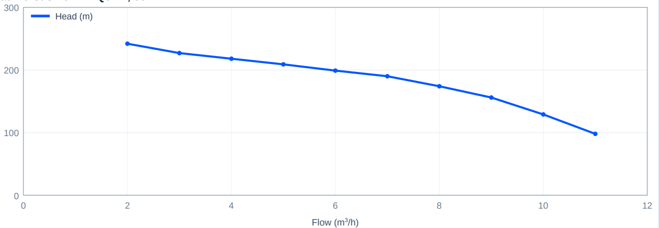
Head versus flow - PQ8-44, 50 Hz
