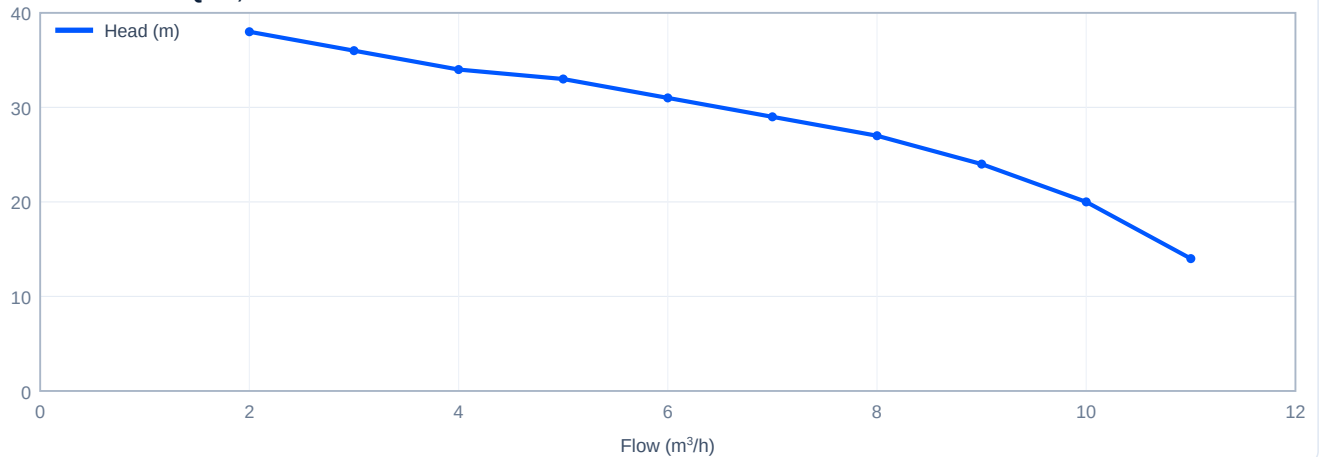
Head versus flow - PQ8-7, 50 Hz
