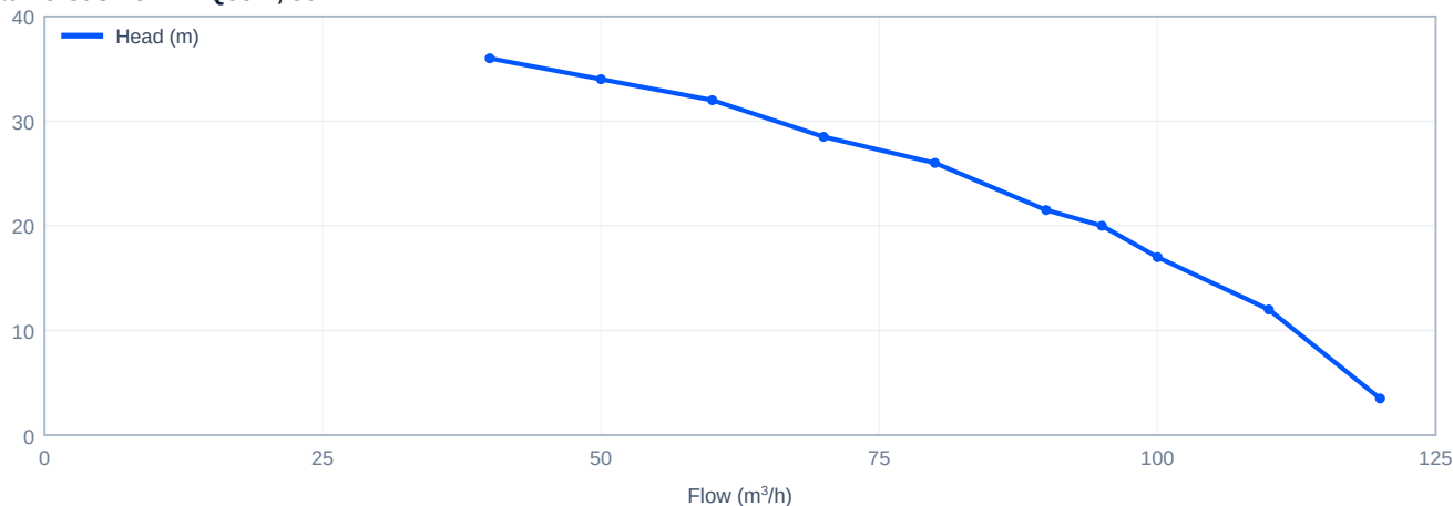
Head versus flow - PQ95-2, 50 Hz
