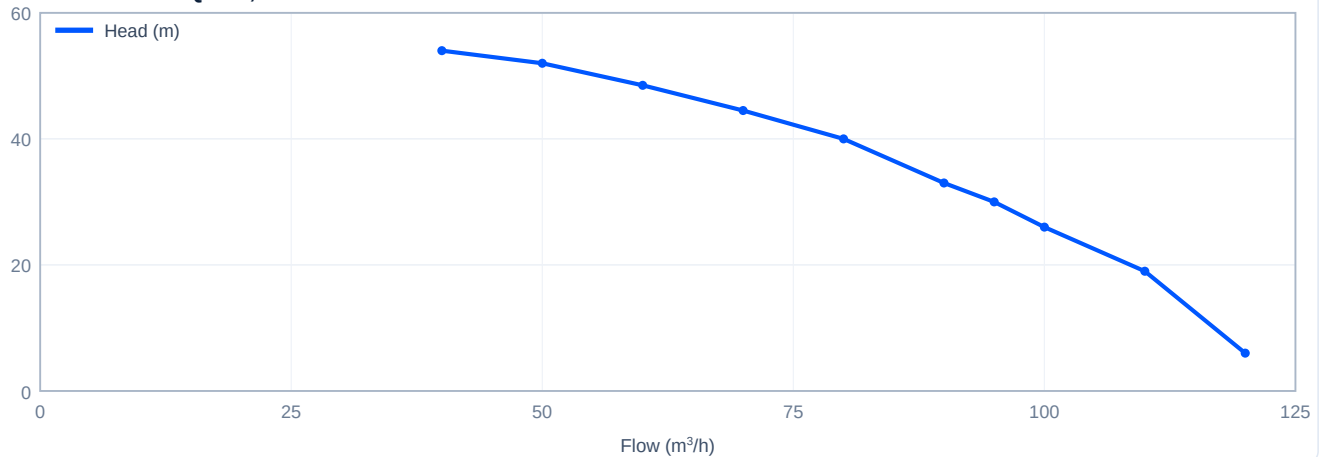
Head versus flow - PQ95-3, 50 Hz
