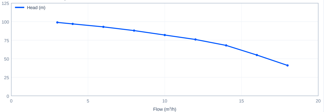
Head versus flow - SJ12-15, 50 Hz
