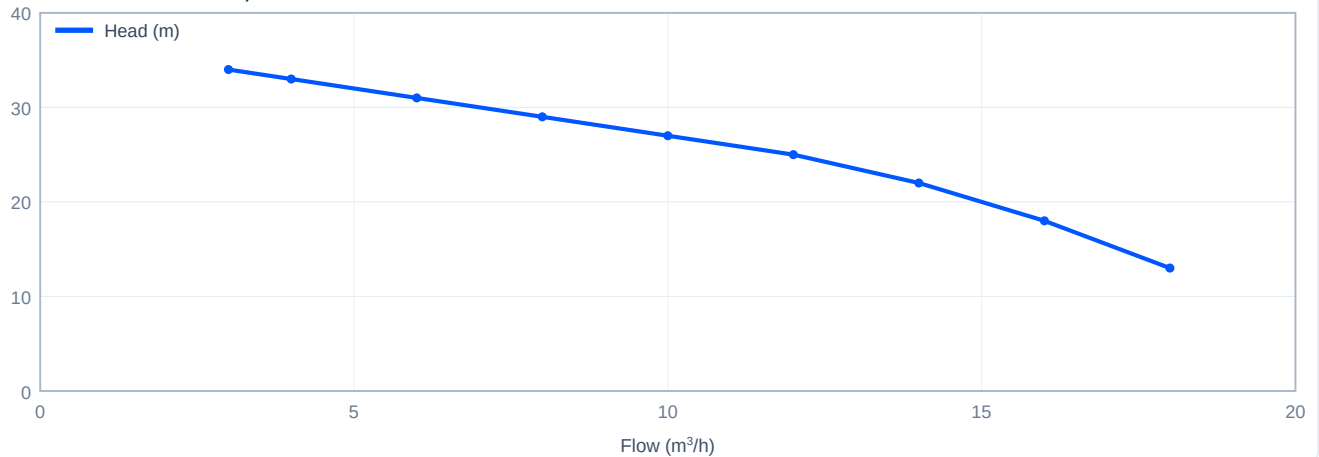
Head versus flow - SJ12-5, 50 Hz
