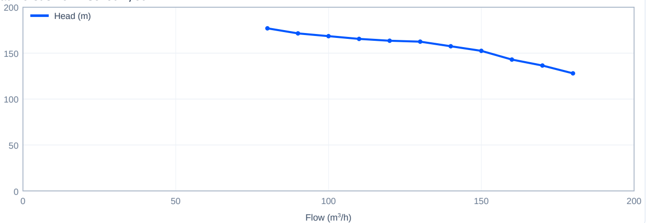
Head versus flow - SJ150-7, 50 Hz
