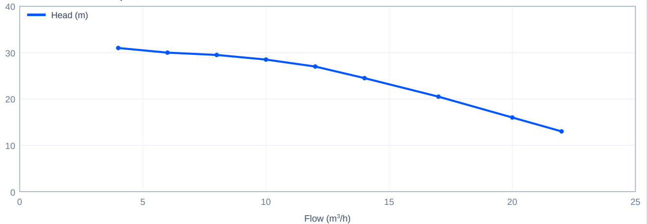
Head versus flow - SJ17-3, 50 Hz
