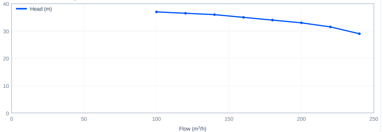
Head versus flow - SJ200-1, 50 Hz
