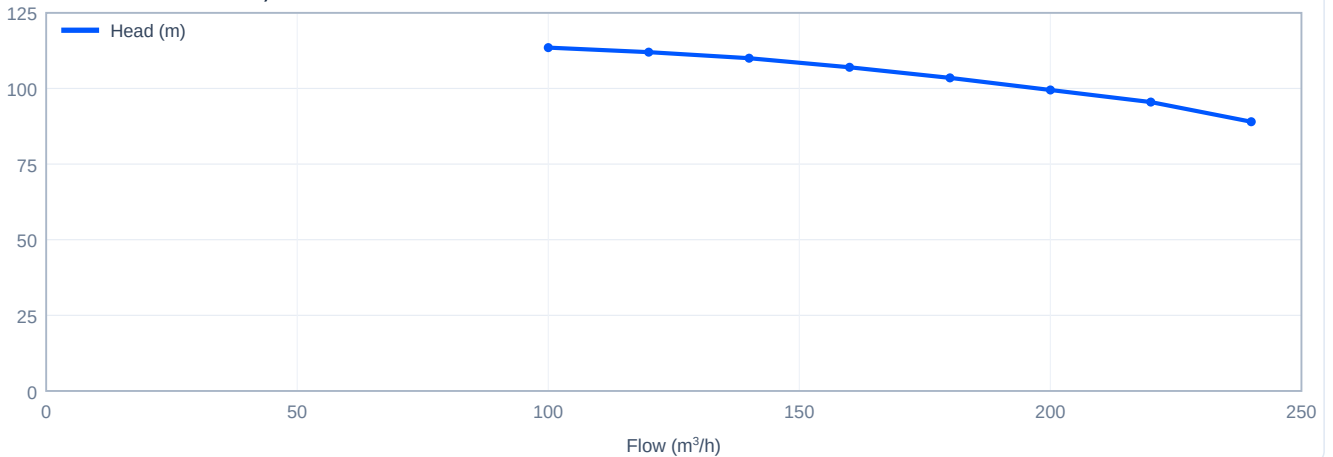
Head versus flow - SJ200-3, 50 Hz
