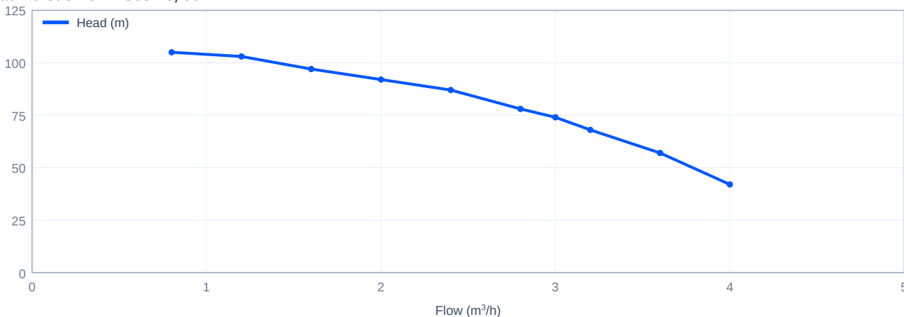
Head versus flow - SJ3-18, 50 Hz
