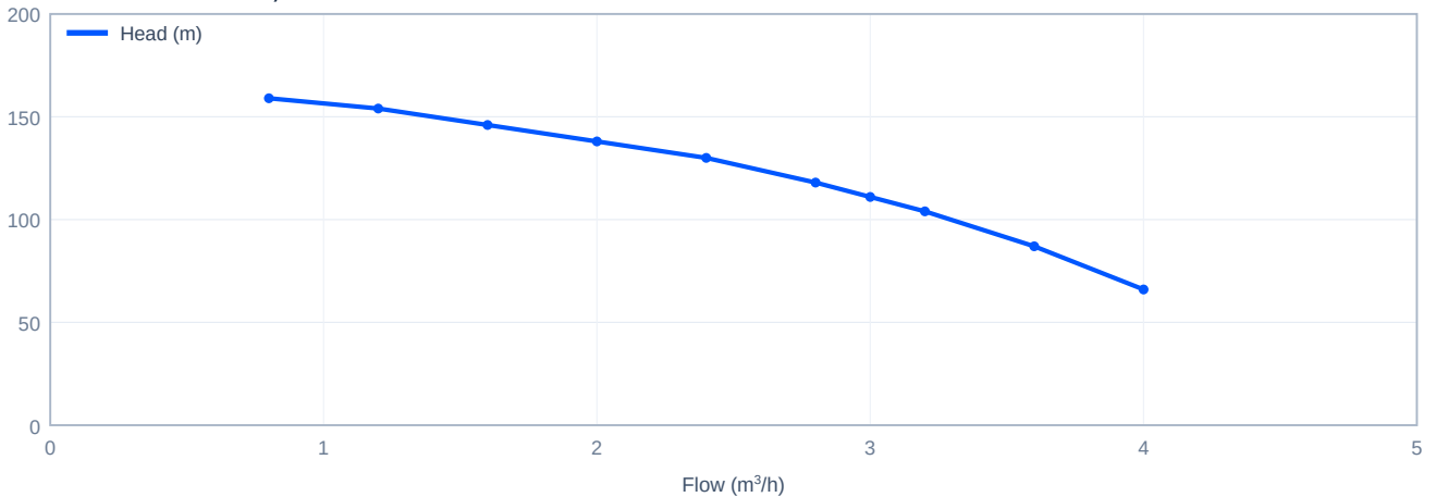
Head versus flow - SJ3-27, 50 Hz
