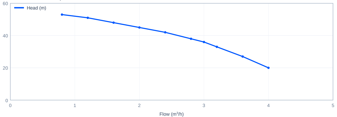
Head versus flow - SJ3-9, 50 Hz
