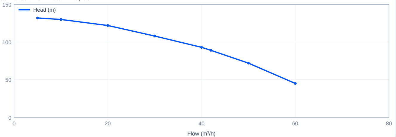
Head versus flow - SJ42-10, 50 Hz
