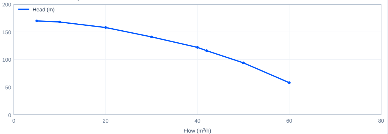
Head versus flow - SJ42-13, 50 Hz
