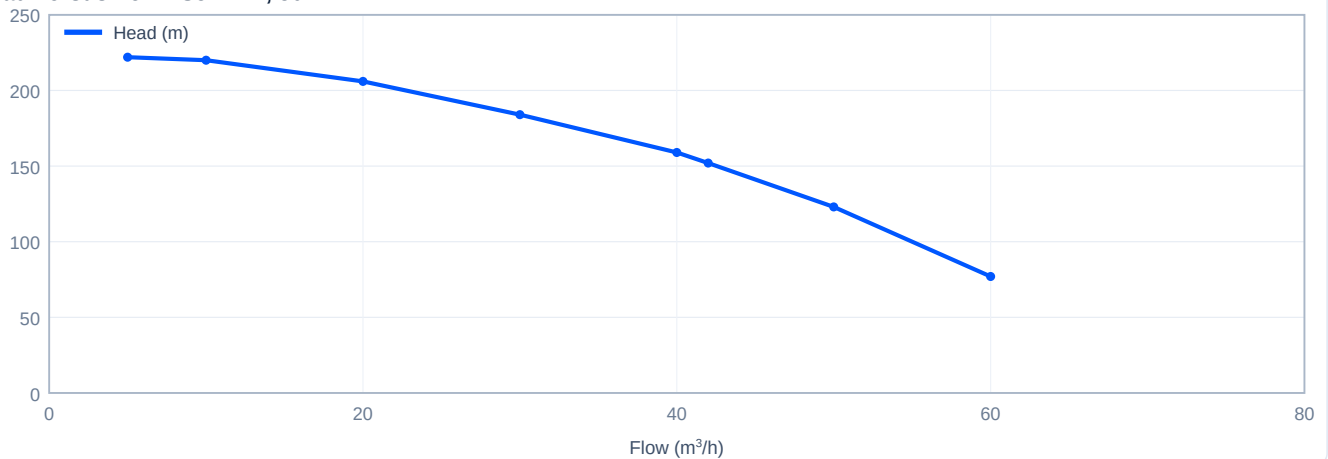
Head versus flow - SJ42-17, 50 Hz
