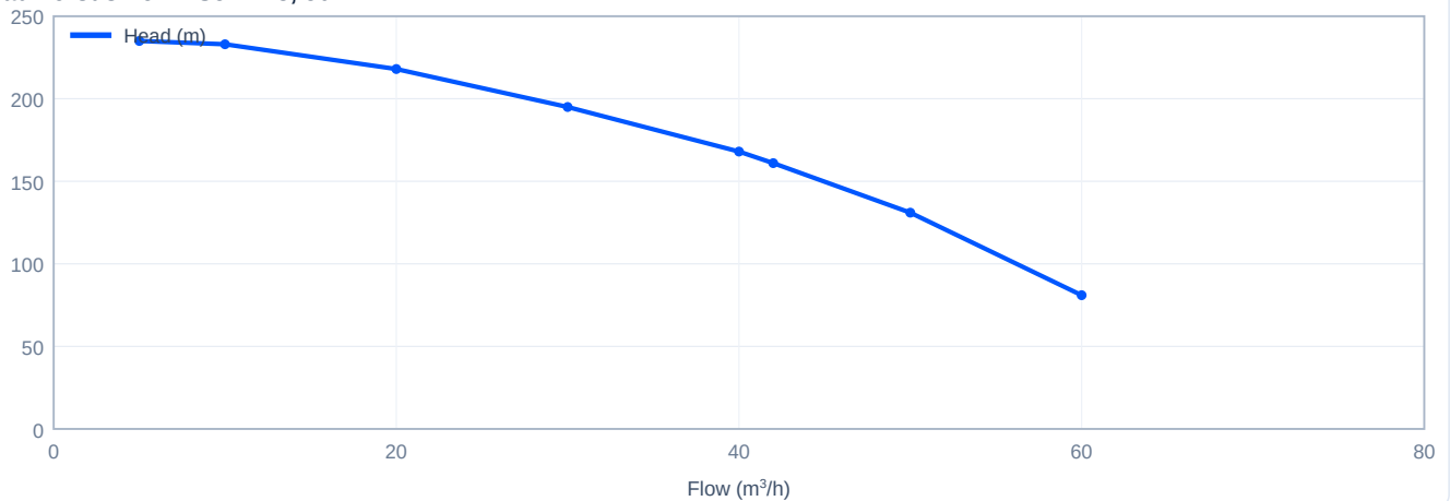
Head versus flow - SJ42-18, 50 Hz
