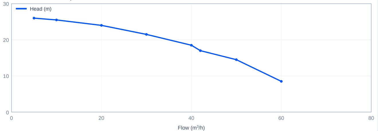
Head versus flow - SJ42-2, 50 Hz
