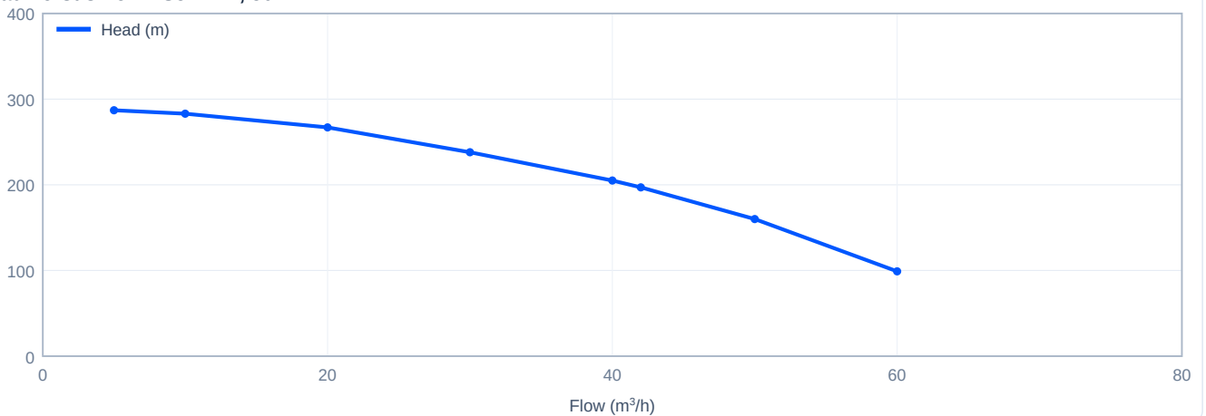
Head versus flow - SJ42-22, 50 Hz
