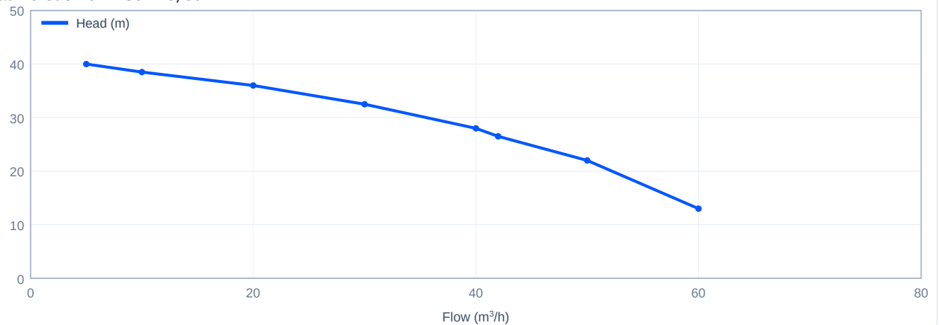
Head versus flow - SJ42-3, 50 Hz
