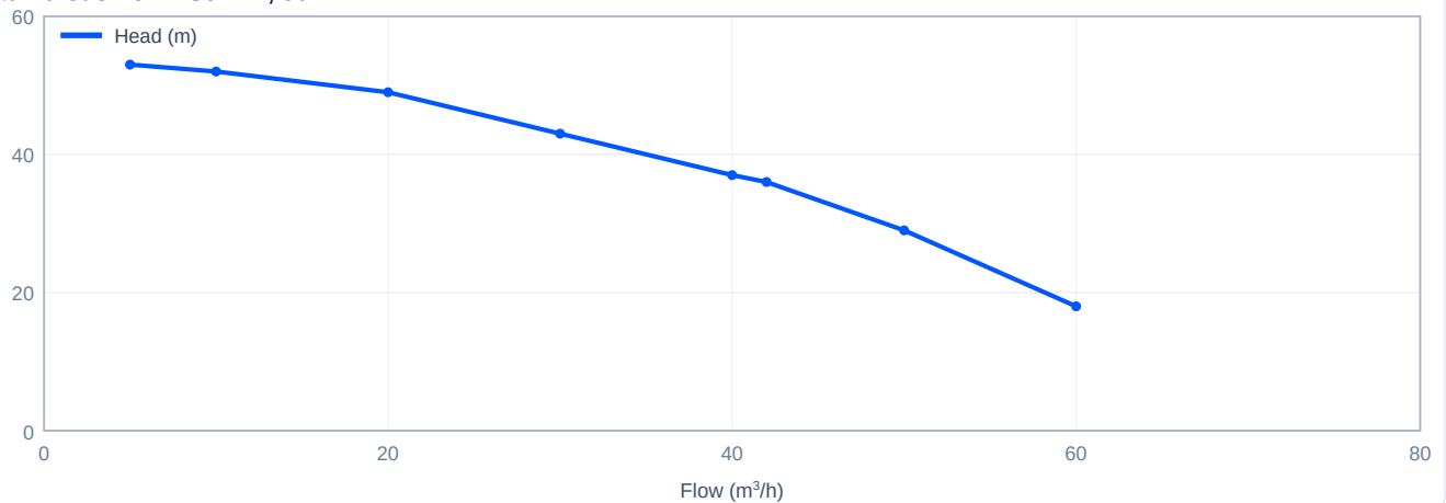
Head versus flow - SJ42-4, 50 Hz
