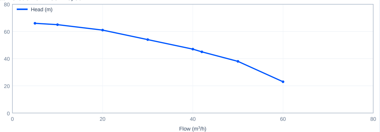
Head versus flow - SJ42-5, 50 Hz
