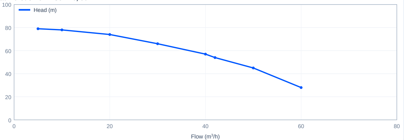
Head versus flow - SJ42-6, 50 Hz
