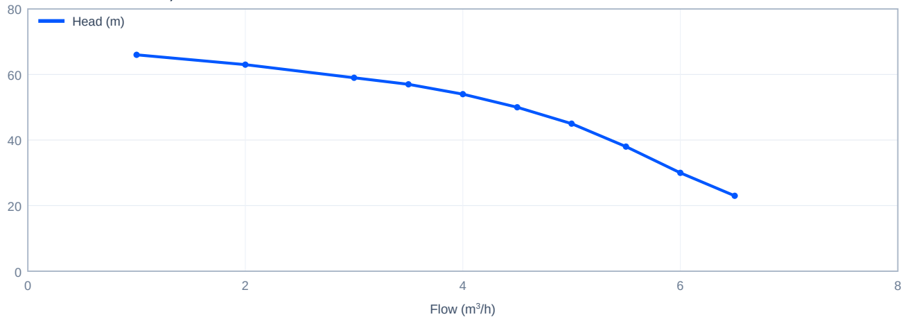
Head versus flow - SJ5-12, 50 Hz
