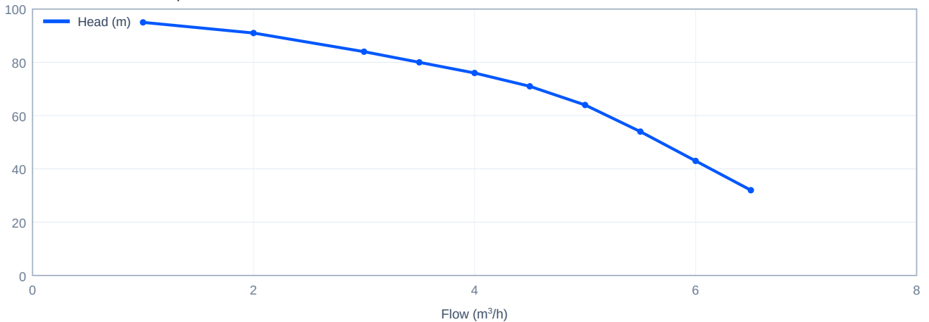
Head versus flow - SJ5-17, 50 Hz
