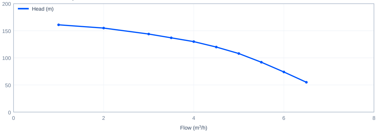
Head versus flow - SJ5-29, 50 Hz
