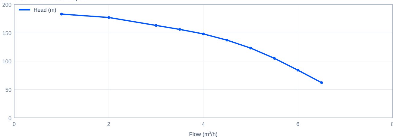
Head versus flow - SJ5-33, 50 Hz
