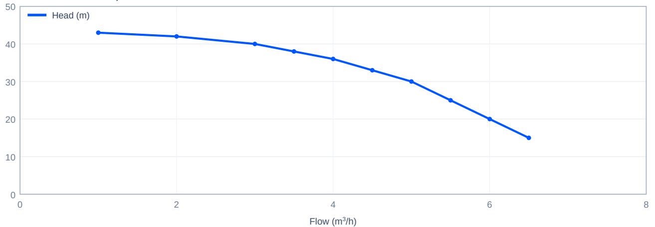
Head versus flow - SJ5-8, 50 Hz
