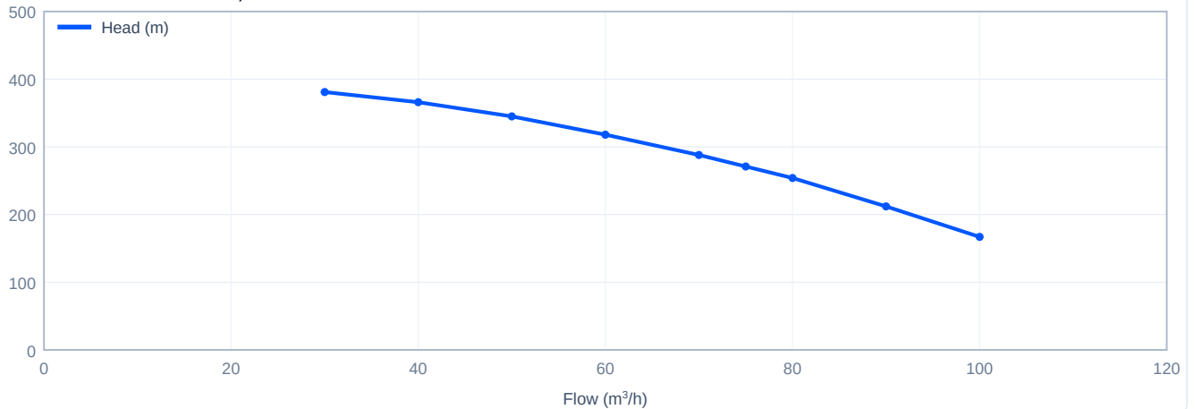
Head versus flow - SJ75-20, 50 Hz
