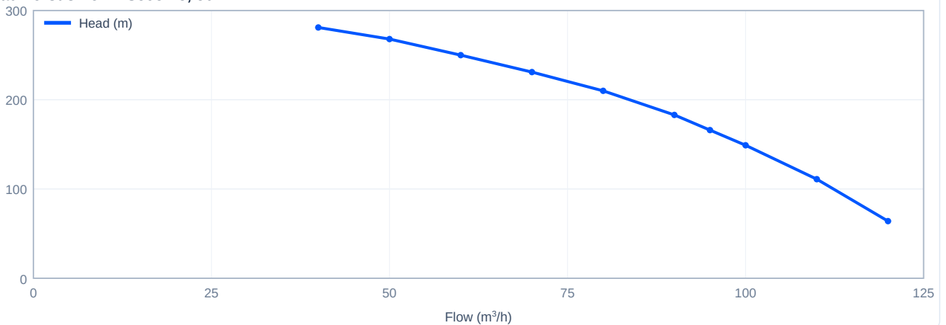
Head versus flow - SJ95-15, 50 Hz
