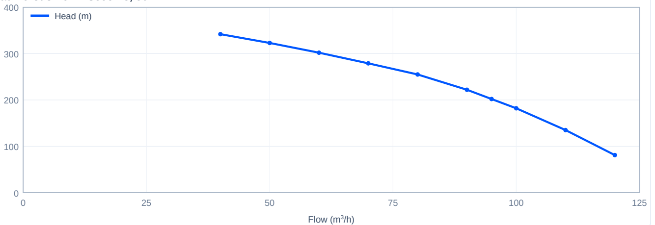
Head versus flow - SJ95-18, 50 Hz
