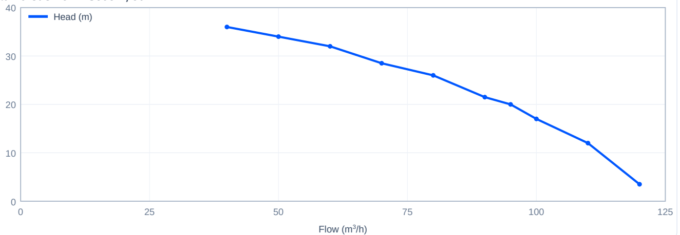
Head versus flow - SJ95-2, 50 Hz
