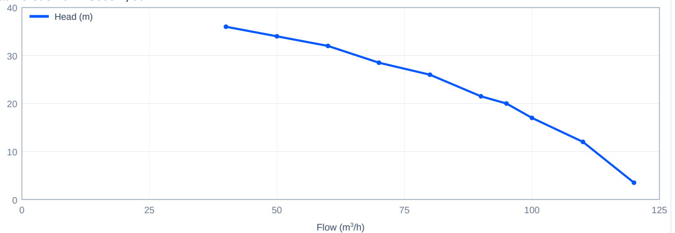
Head versus flow - SJ95-2, 50 Hz
