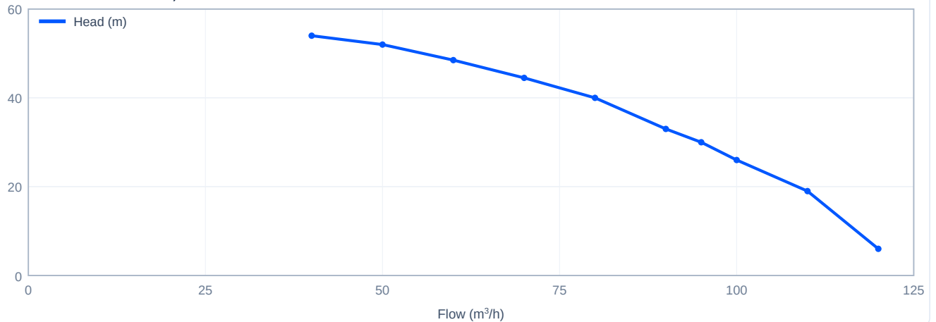
Head versus flow - SJ95-3, 50 Hz
