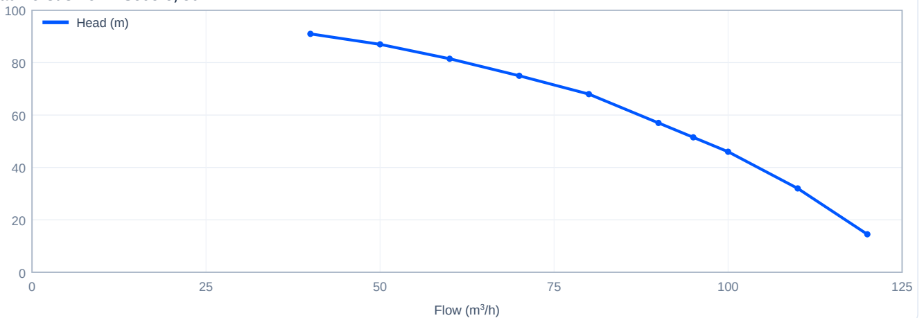
Head versus flow - SJ95-5, 50 Hz
